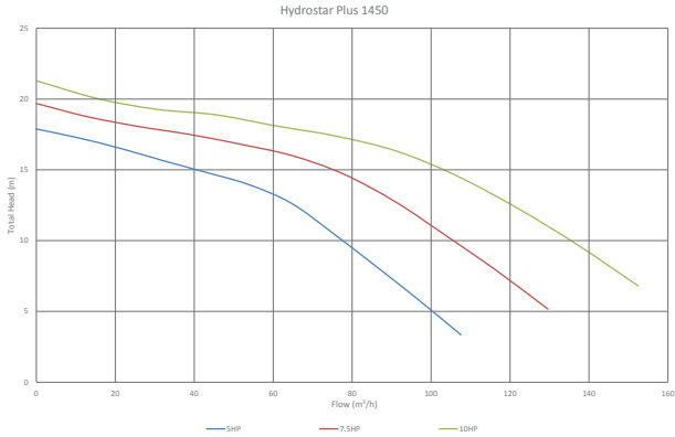
Flow Curve
