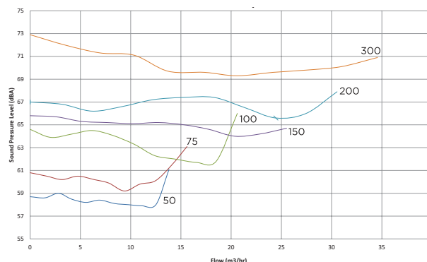
Noise Curve
