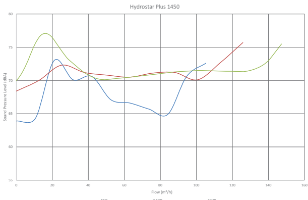
Noise Curve
