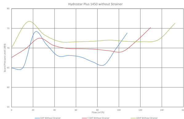
Noise Curve
